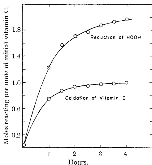
Fig. 2.—Reaction between vitamin C and hydrogen peroxide.
